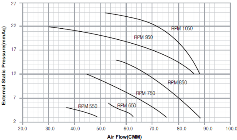
◆ Fan Performance (ARNU76GB8A4, ARNU96GB8A4)
